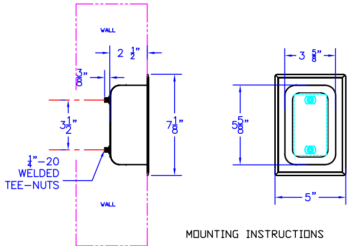
HORIZONTAL MOUNT
